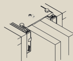
Connector 110 mm (4 11/32"): Recess for two pivot/slide-in doors.
